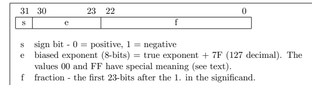
Figure 6.3: IEEE single precision
