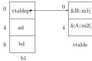
Figure 7.24: Internal representation of b1
