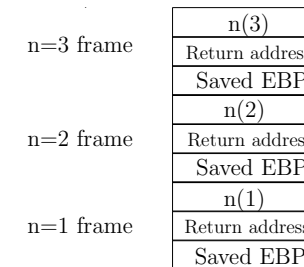
Figure 4.16: Stack frames for factorial function
