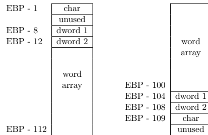
Figure 5.2: Arrangements of the stack
